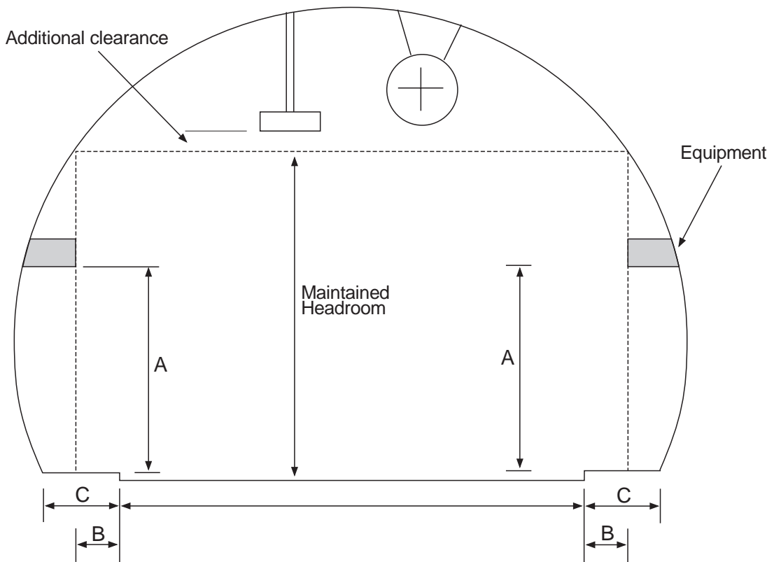
Figure 4.2 Example Arch Profile
