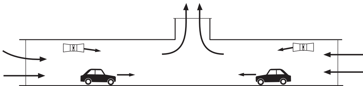
Longitudinal Ventilation with Central Exhaust Shaft (Two way traffic - Long tunnel)
