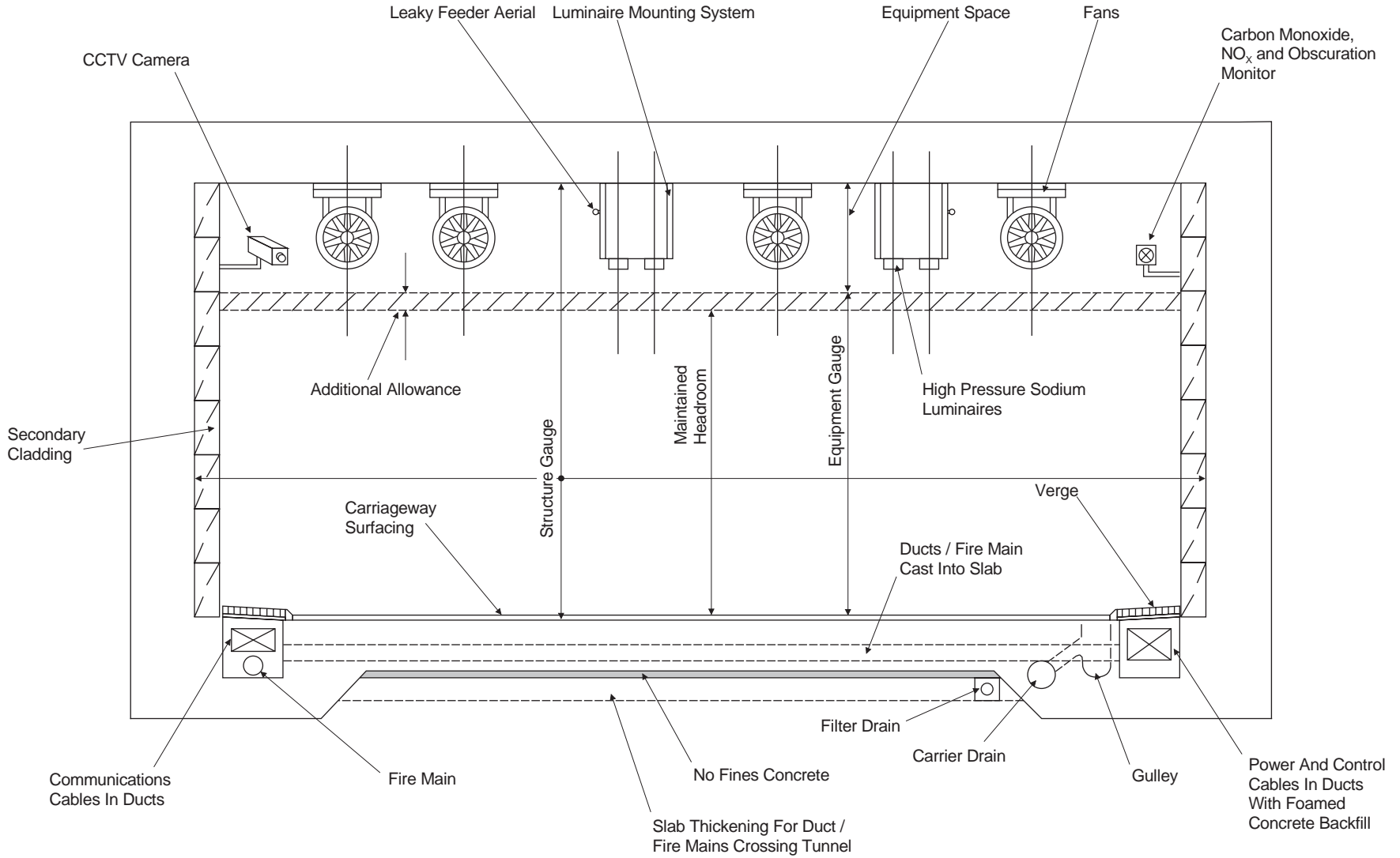
Typical Cut and Cover Tunnel Section (Looking In Direction Of Traffic Flow)
